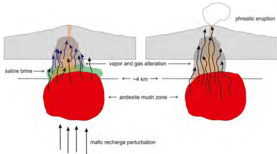
Figure 4. Preeruption and posteruption systems. The red chamber is the andesite partial melt reservoir; green the brine lens; blue arrows represent vapor (saline) coming off the brine; black arrows are gas exsolving from the magma creating the zone of alteration around the conduit (C2 in Figure 3a). Mafic recharge or an alternate perturbation of the andesite reservoir mobilizes the melt allowing it to reach the overlying brine triggering the phreatic eruption. Dashed line is ~4 km below surface.
