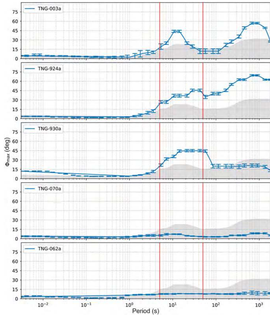
Figure 2. Plot showing the difference phase tensor property \Phi_{\max} between preeruption and posteruption observations. The gray background is the estimated noise tensor difference (i.e., the change in observed response that can be attributed solely to measurement noise). The two stations distal to the eruption center (062 and 070) show no significant change. Three representative sites overlying the magmatic system (003, 924, and 930) show a clear change above the estimated error for the periods 5–50 s (red) corresponding to the \sim depth range of C1.
