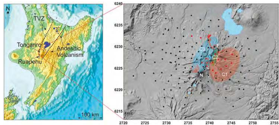
Figure 1. Magnetotelluric site locations (New Zealand Map Grid coordinate system) showing the location of the major features of the resistivity model: C1 = the reservoir (red), C2 = conduit (green), and C3 = near-surface hydrothermal system (blue), also shown in Figure 3a. Seismic activity preceding the 2012 eruptions was located within the crosshatched black ellipsoid. Both the original preeruption survey (black) and repeated posteruption (red) locations are shown. Extrusive lava flows from the Te Mari (T) and Ngauruhoe (N) vents are also shown. The left panel shows the survey area relative to the major andesitic volcanic cones of the southern Taupo Volcanic Zone.
