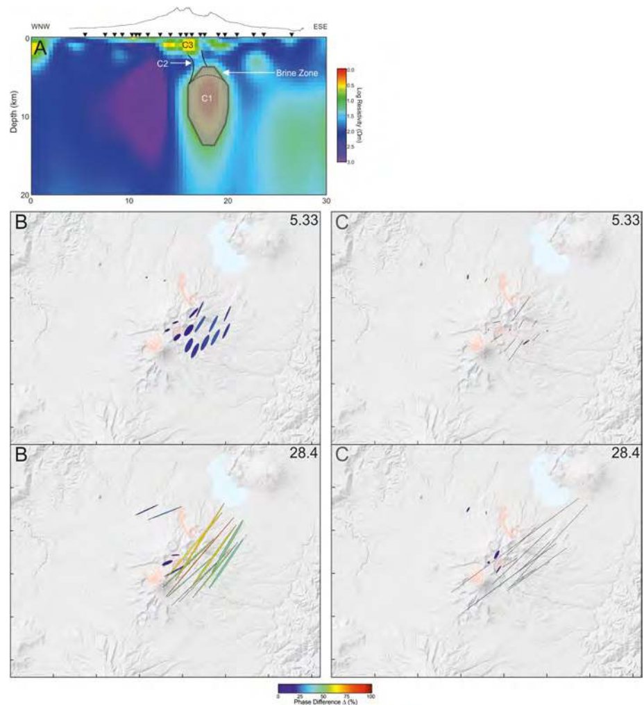
Figure 3. Difference ellipses. (a) Preeruption cross section showing the preeruption reservoir C1 where the resistivity was varied. (b) Synthetic difference ellipses when the resistivity of C1 has been increased to 15 \Omega\text{m} and the brine layer removed which best reproduce the magnitude and direction of the observed difference tensor. (c) Observed difference ellipses (as the change is highly polarized the ellipse minor axis is small leading to the narrow shape) at two periods (5.33 and 28.4 s) showing the first onset of differences above 7% at 5.33 s and the highly polarized (represented by the elongate ellipse) nature of the change at 28.4 s. Note difference tensor ellipses are plotted at 4 times scale of those in supporting information Figure S1.
